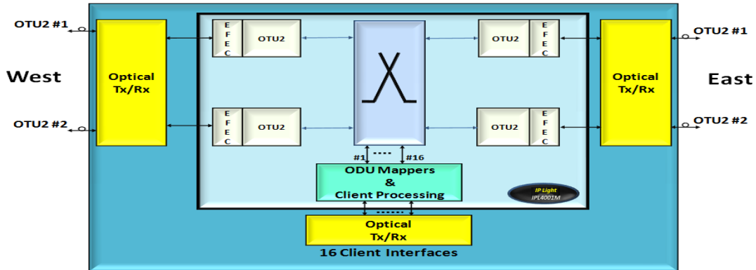
Figure 14: Single-Chip two OTU2 rings ADM with Drop/Insert of 40Gbps of Client traffic
